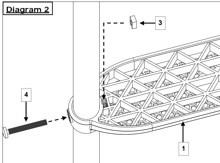
(Under side of step, showing square nut location)
