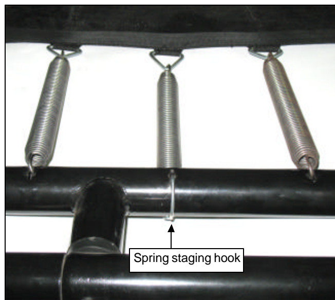
(Overview showing proper installation of a completed SB2 Spring Staging System)
